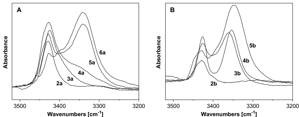
Figure 8. FTIR absorption spectra in the N–H stretching region of the ( R )-Bip[( S )Binol-22-C-6]/L-Ala peptide series 2a–6a (A) and the ( R )-Bip[( S )Binol-22-C-6]/L-Ala/Aib series 2b–5b (B) in CDCl 3 solution (peptide concentration: 1 mM).
