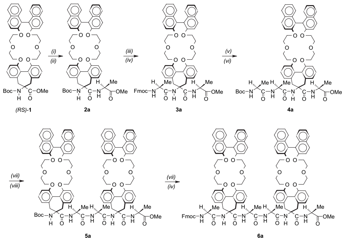
Figure 6. Synthesis of peptides based on ( R )-Bip[( S )-Binol-22-C-6] combined with L-Ala ( a series). (i) 1 N NaOH, MeOH, 50 °C; (ii) HCl·H-L-Ala-OMe, HATU, DIEA, CH 2 Cl 2 /THF; (iii) TFA/CH 2 Cl 2 1:3; (iv) Fmoc-L-Ala-NCA, DIEA, THF; (v) 10% (v/v) Et 2 NH/CH 3 CN–CH 2 Cl 2 ; (vi) Boc-L-Ala-OH, EDC, HOAt, CH 2 Cl 2 ; (vii) HCl/dioxane ≈ 4 N, CH 2 Cl 2 ; (viii) Boc-( R )-Bip[( S )-Binol-22-C-6]-OH, HATU, DIEA, CH 2 Cl 2 /THF.
