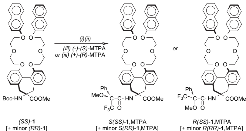
Figure 4. Synthesis of the diastereomeric Mosher's amides S ( SS )-1, MTPA and R ( SS )-1, MTPA from ( SS )-1. (i) TFA/CH 2 Cl 2 1:3, 0 °C to rt; (ii) EDC, CH 3 CN, rt.
