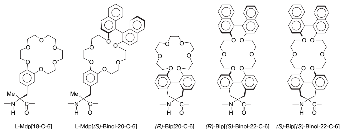
Figure 1. Chemical structures of L-Mdp[18-C-6], L-Mdp[(S)-Binol-20-C-6], (R)-Bip[20-C-6], (R)-Bip[(S)-Binol-22-C-6], and (S)-Bip[(S)-Binol-22-C-6] residues.
