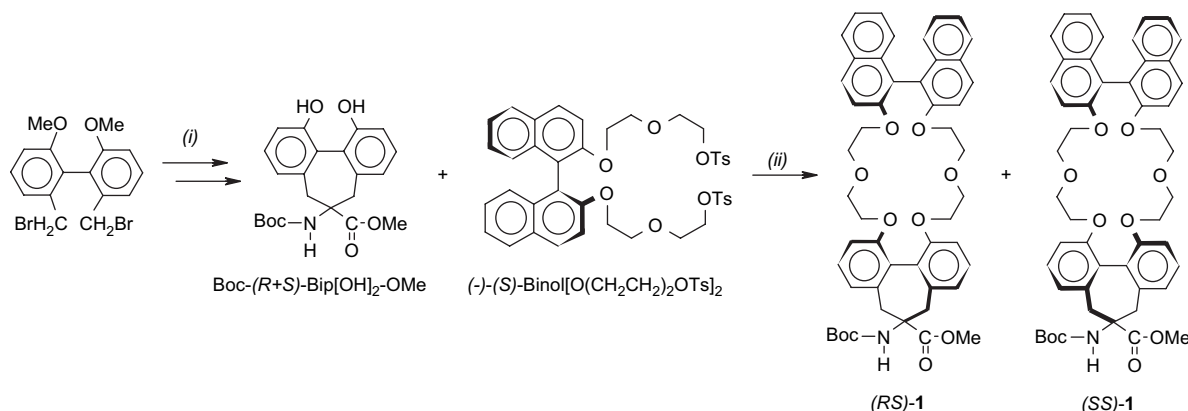
Figure 2. Synthesis of Boc-( R )-Bip[( S )-Binol-22-C-6]-OMe ( RS )-1 and Boc-( S )-Bip[( S )-Binol-22-C-6]-OMe ( SS )-1. (i) Ref. 36; (ii) Cs 2 CO 3 ; DMF; 60 °C.
