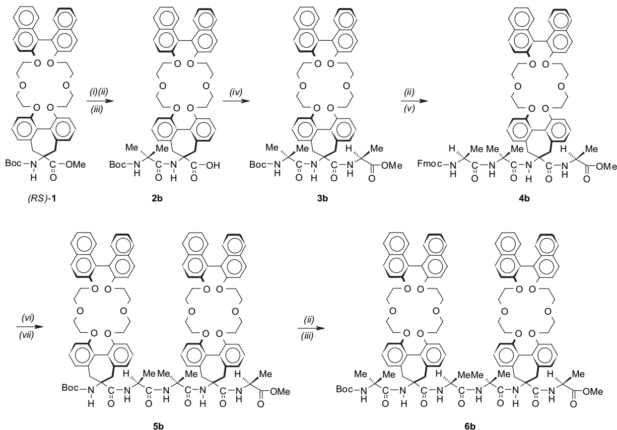
Figure 7. Synthesis of peptides based on ( R )-Bip[( S )-Binol-22-C-6] combined with L-Ala and Aib ( b series). (i) 1 N NaOH, MeOH, 50 °C; (ii) TFA/CH 2 Cl 2 1:3; (iii) Boc-Aib-NCA, DIEA, THF; (iv) HCl·H-L-Ala-OMe, HATU, DIEA, CH 2 Cl 2 /THF; (v) Fmoc-L-Ala-NCA, DIEA, THF; (vi) 10% (v/v) Et 2 NH/CH 2 Cl 2 ; (vii) Boc-( R )-Bip[( S )-Binol-22-C-6]-OH, HATU, DIEA, CH 2 Cl 2 /THF.
