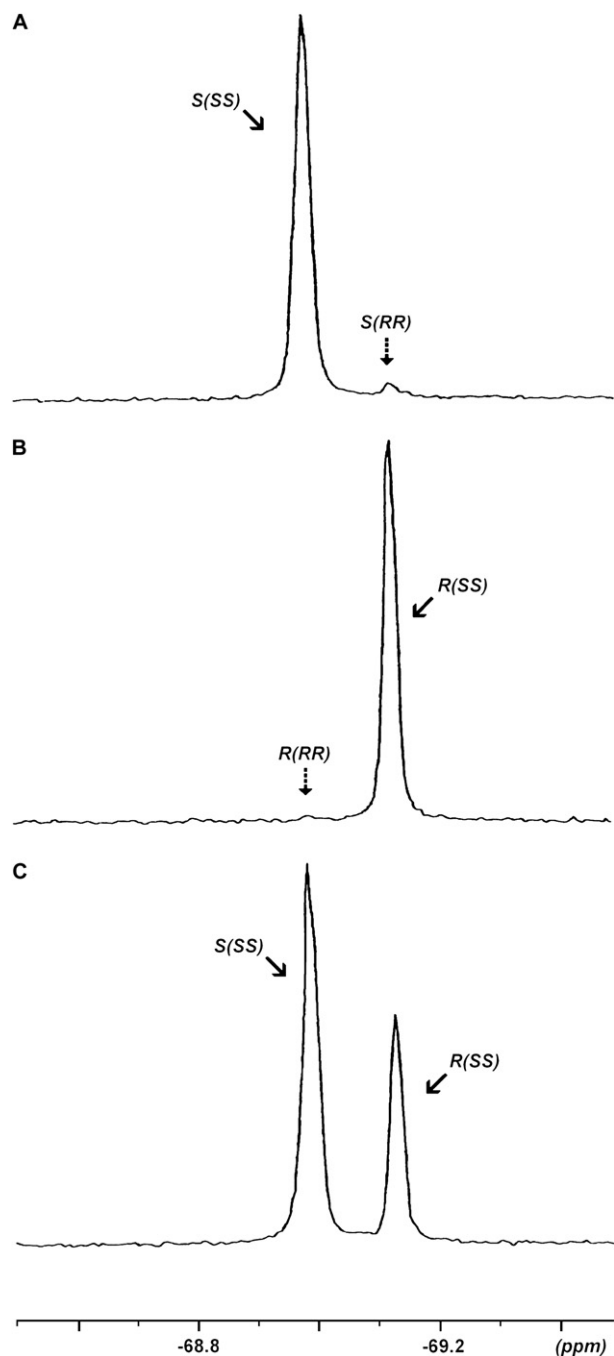
Figure 5. ^{19}\text{F} NMR spectra of the Mosher's amido esters S(SS) - 1 , MTPA ( A ) and R(SS) - 1 , MTPA ( B ) in toluene- d_8 solution, as compared to the spectrum of an artificial mixture of both solutions of S(SS) - 1 , MTPA (major) and R(SS) - 1 , MTPA (minor) ( C ).
