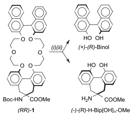
Figure 3. Cleavage of the postulated ( RR )-1 isomer to (+)-( R )-Binol and (–)-( R )-H-Bip[OH] 2 -OMe. (i) BBr 3 , CH 2 Cl 2 , –10 °C to rt; (ii) MeOH, SOCl 2 , rt.
