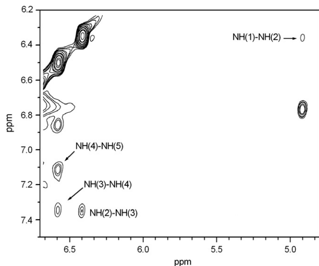
Figure 9. Section of the ROESY spectrum of the ( R )-Bip[( S )Binol-22-C-6]/L-Ala pentapeptide 5a in CDCl 3 solution (peptide concentration: 1 mM) showing the NH( i )→NH( i +1) connectivities.
